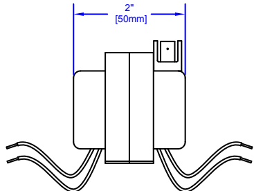
CX-TRX-2024 - 24VAC, 40 VA STANDARD MOUNT TRANSFORMER
