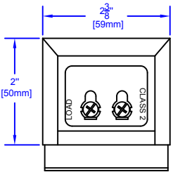
CX-TRX-2012 12VAC 20VA NIPPLE MOUNT TRANSFORMER.
