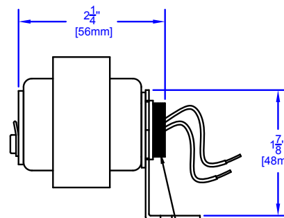
CX-TRX - 2012 12VAC 20VA NIPPLE MOUNT TRANSFORMER.
