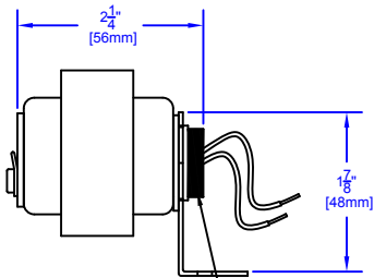
CX-TRX-2012 12VAC 20VA NIPPLE MOUNT TRANSFORMER.
