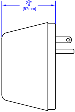
CX-TRP-4016 - 16VAC, 40 VA Plug-in transformer
