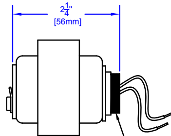
CX-TRN - 2024 - 24V AC 20VA NIPPLE MOUNT TRANSFORMER
