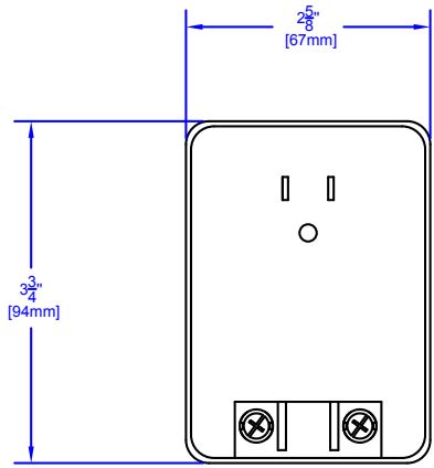
CX-TRP-4016 - 16VAC, 40 VA Plug-in transformer
